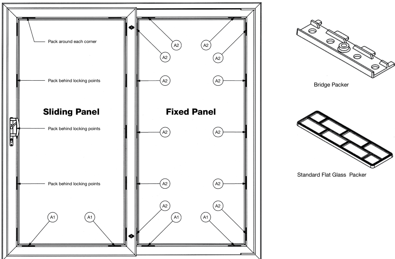
Fig. 2.0: Packing points illustrated. Packer positions are made up of a combination of Bridge packer and a suitable number of flat packers (as required). Repeat packing procedure on sliding panel.
